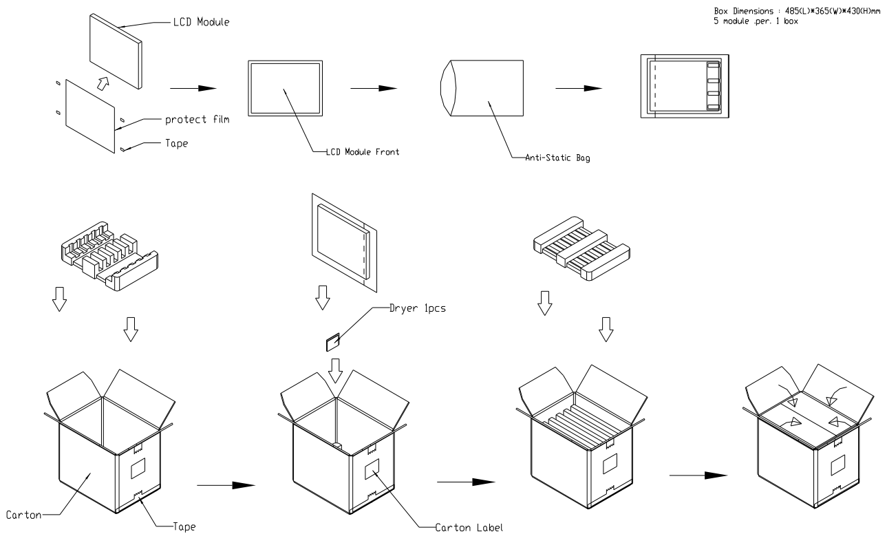
Figure. 7-1 Packing method
