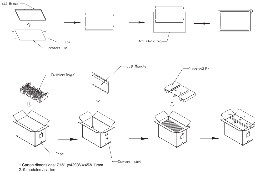
Figure. 7-1 Packing method
