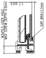
SECTION USER_HOLE--USER_HOLE SCALE 4:1
