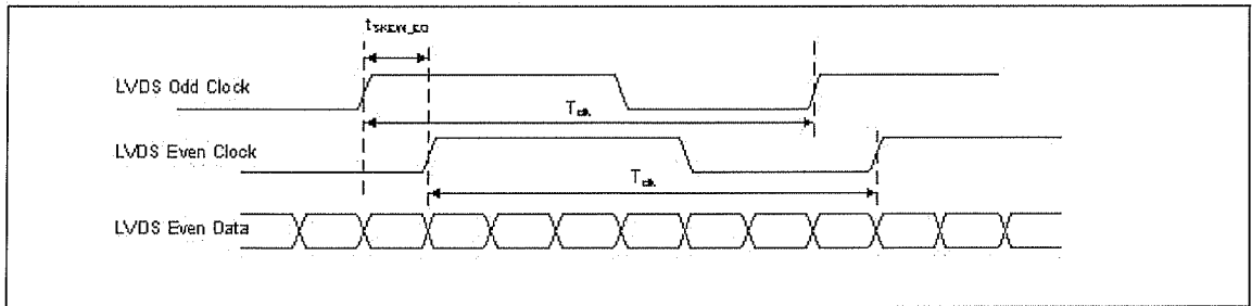
< Clock skew margin between channel >
