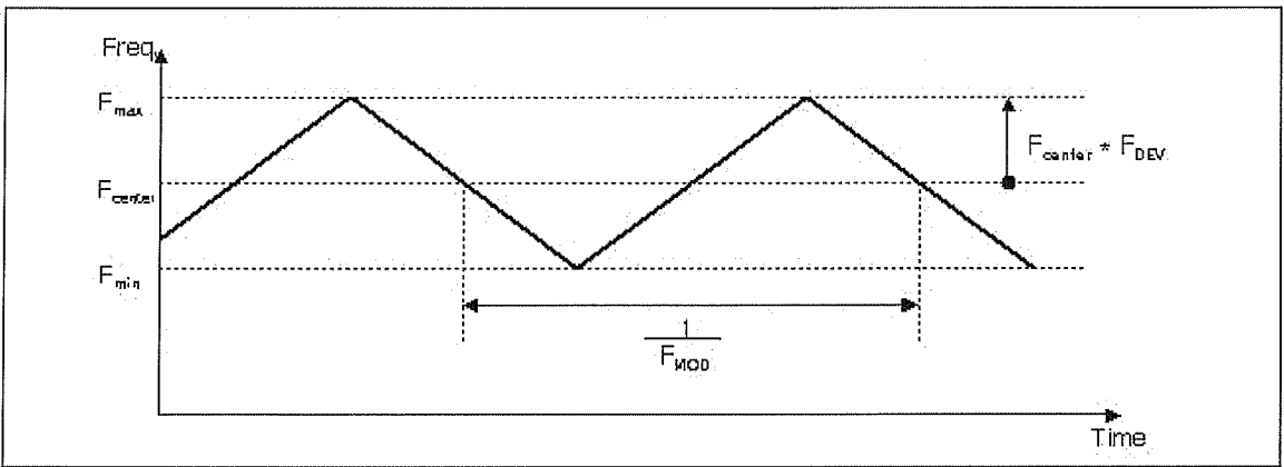
< Spread Spectrum >
