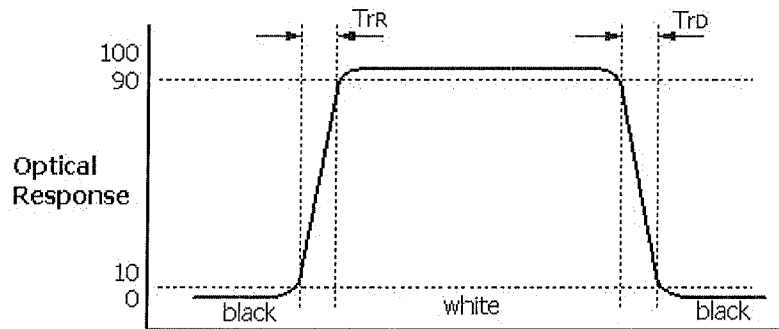
FIG. 8 Response Time
